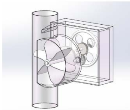
Fig.3. Power generation part
